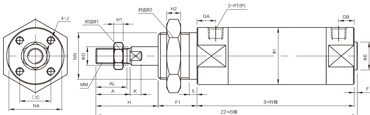
DHR1P尺寸图
