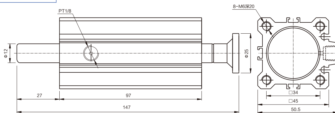
DHR2H32N20Z尺寸图
