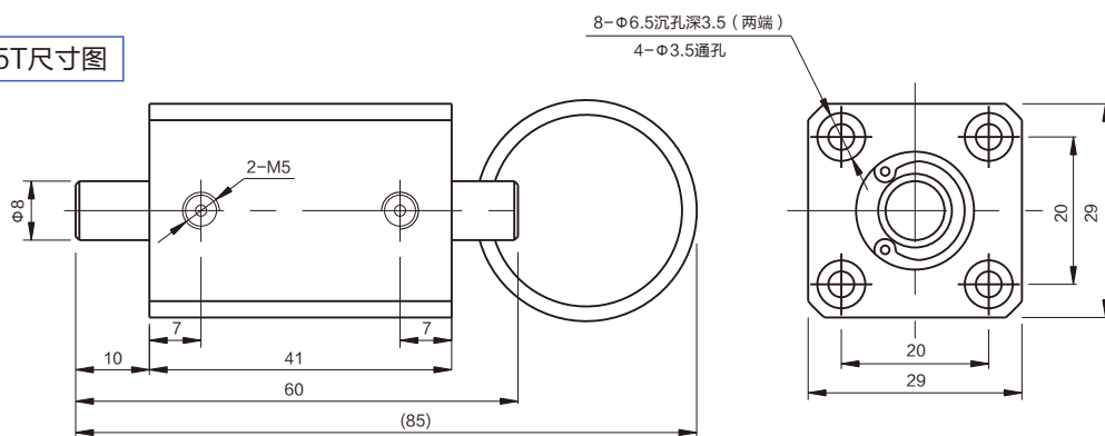
DHR2H20N15Z尺寸图
